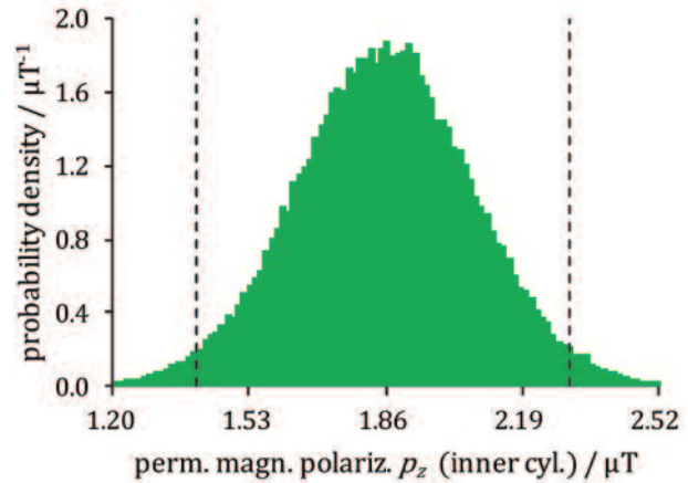
Figure 13: Scaled frequency distribution of the permanent magnetic polarization p_z after the approximation with the inner cylinders. The dashed vertical lines give the endpoints of the probabilistically symmetric 95.45 % coverage interval [10]
