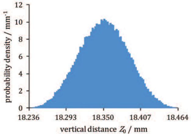
Figure 5: Scaled frequency distribution of the vertical distance Z_0^{\min}
