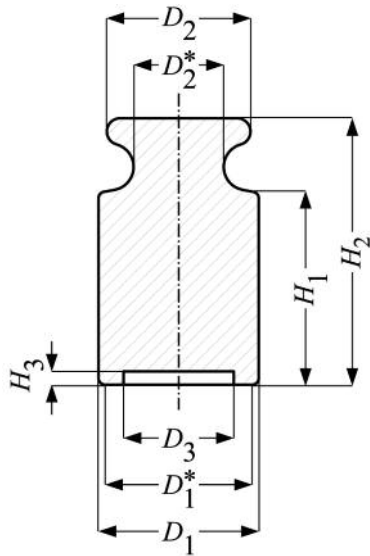
Figure 2: Schematic cross section of a cylindrical weight with a recessed base according to OIML R 111 [3]
