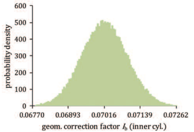
Figure 9: Scaled frequency distribution of the geometrical approximation factor I_b after the approximation with the inner cylinders
