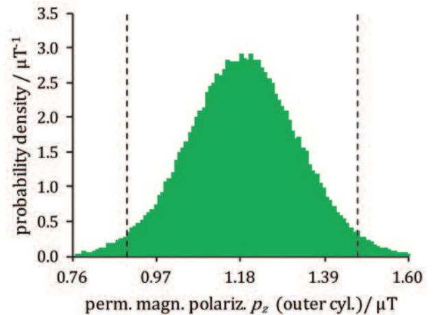
Figure 11: Scaled frequency distribution of the permanent magnetic polarization p_z after the approximation with the outer cylinders. The dashed vertical lines give the endpoints of the probabilistically symmetric 95.45 % coverage interval [10]
