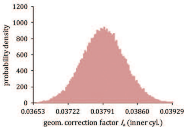
Figure 8: Scaled frequency distribution of the geometrical approximation factor I_a after the approximation with the inner cylinders
