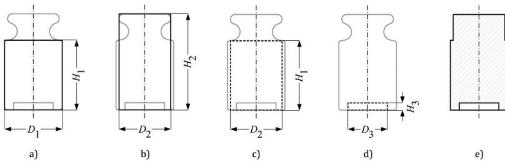
Figure 3: Illustration of the geometrical approximation of an OIML weight in an upright position with "outer" cylinders. a) – d) single cylinders used for the superposition, whereby the dashed cylinders c) and d) have a negative sign; e) schematic cross section of the external shape of an OIML weight after the approximation with outer cylinders [5]
