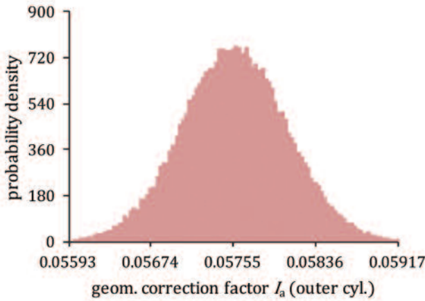
Figure 6: Scaled frequency distribution of the geometrical approximation factor I_a after the approximation with the outer cylinders
