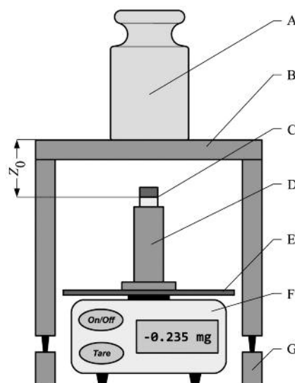
Figure 1: Schematic experimental setup of a susceptometer according to Davis [3-5]
