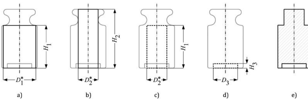
Figure 4: Illustration of the geometrical approximation of an OIML weight in an upright position with "inner" cylinders. a) – d) single cylinders used for the superposition, whereby the dashed cylinders c) and d) have a negative sign; e) schematic cross section of the external shape of an OIML weight after the approximation with inner cylinders [5]
