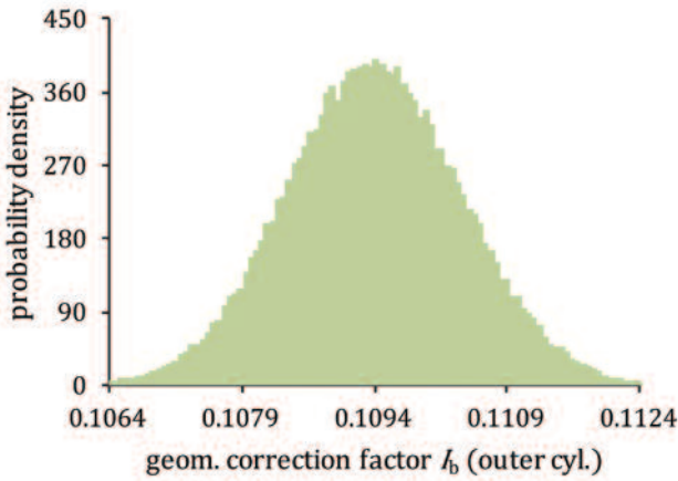
Figure 7: Scaled frequency distribution of the geometrical approximation factor I_b after the approximation with the outer cylinders
