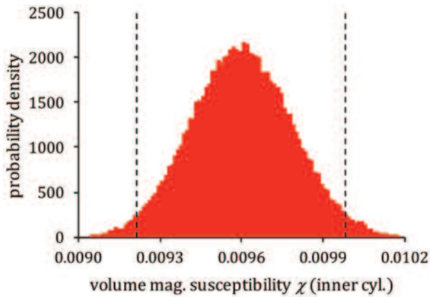
Figure 12: Scaled frequency distribution of the volume magnetic susceptibility \chi after the approximation with the inner cylinders. The dashed vertical lines give the endpoints of the probabilistically symmetric 95.45 % coverage interval [10]
