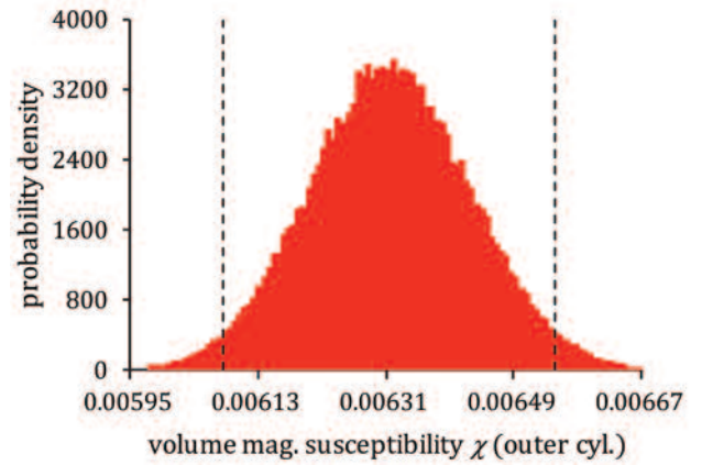
Figure 10: Scaled frequency distribution of the volume magnetic susceptibility \chi after the approximation with the outer cylinders. The dashed vertical lines give the endpoints of the probabilistically symmetric 95.45 % coverage interval [10]
